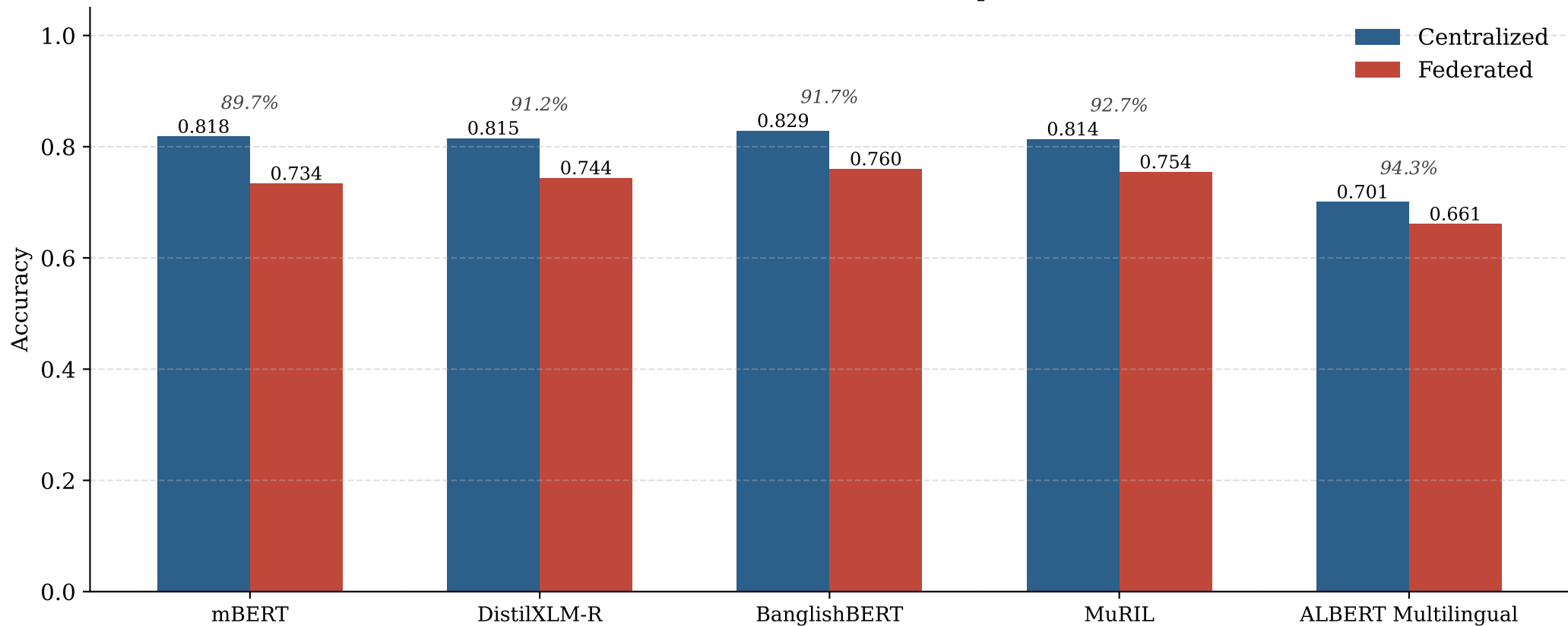
Accuracy Retention: Centralized vs. Federated (all five matched backbone pairs)
